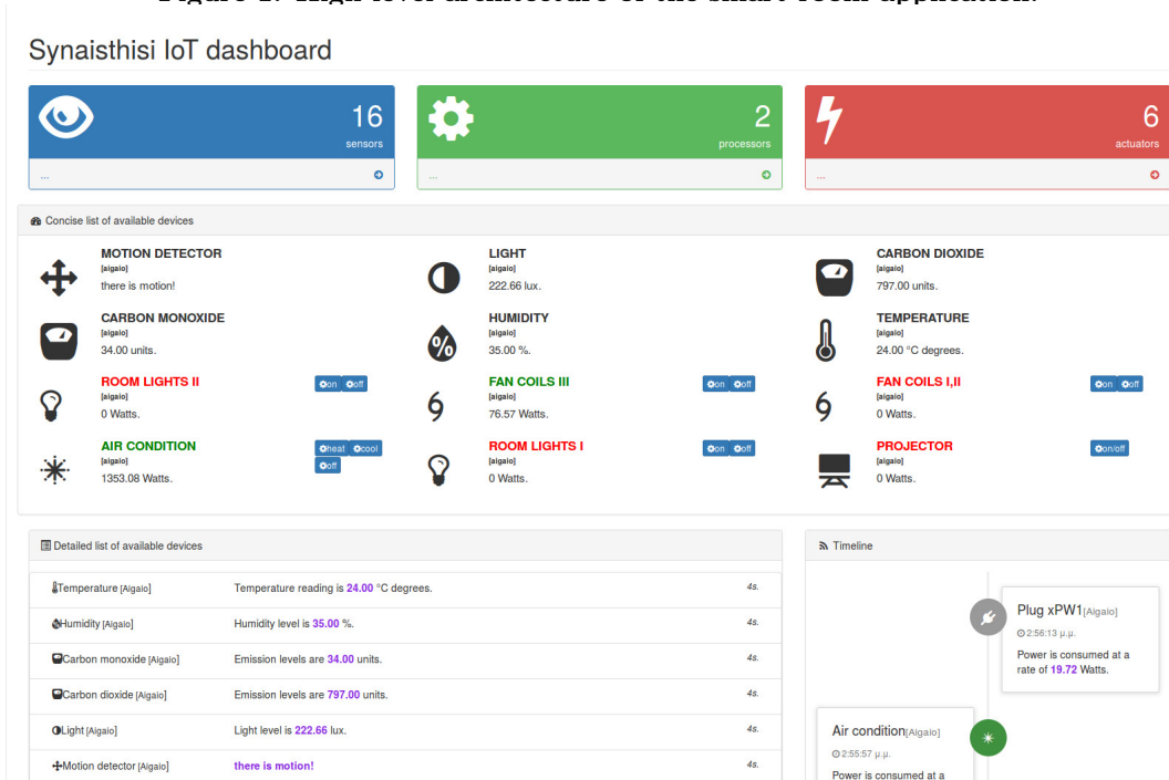
Figure 2: The smart room dashboard offers monitoring and remote control capabilities.
