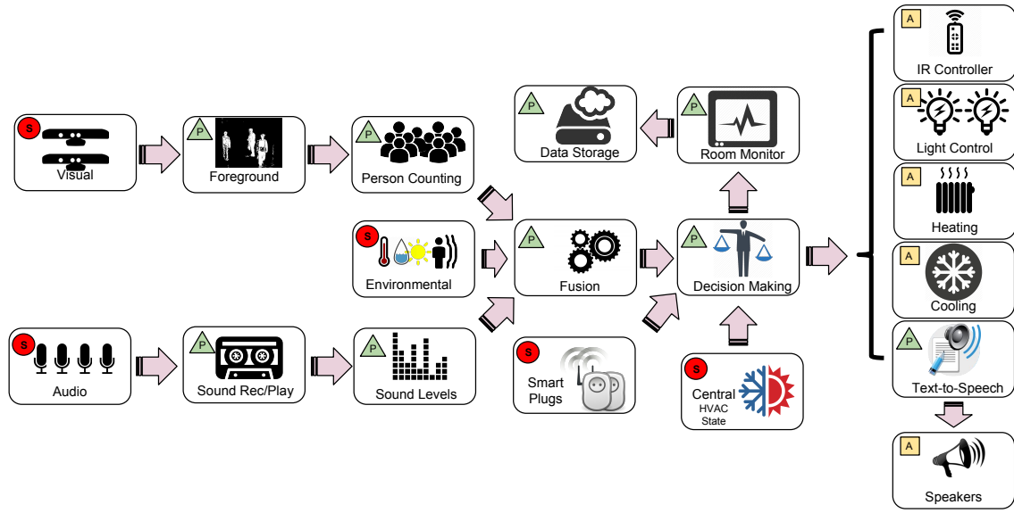
Figure 1: High-level architecture of the smart room application.
